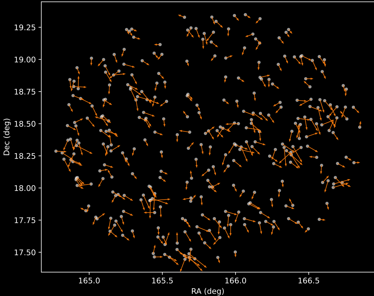
GALAH DR4 Cluster 2 Proper Motion Vectors (n=316)
