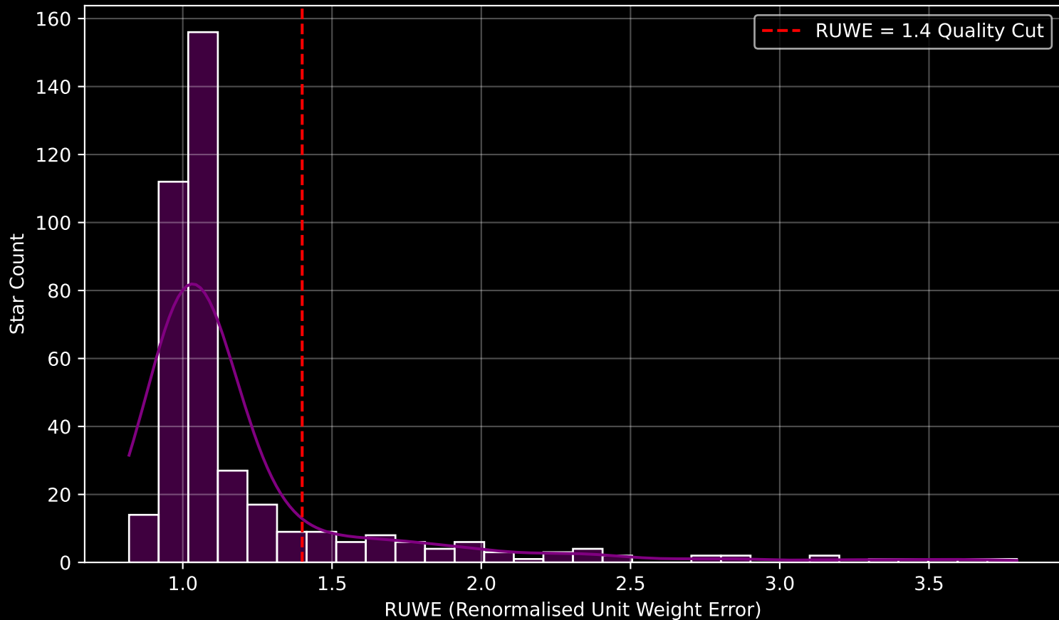
GALAH DR4 Field [6584] RUWE Distribution (n= 398)
