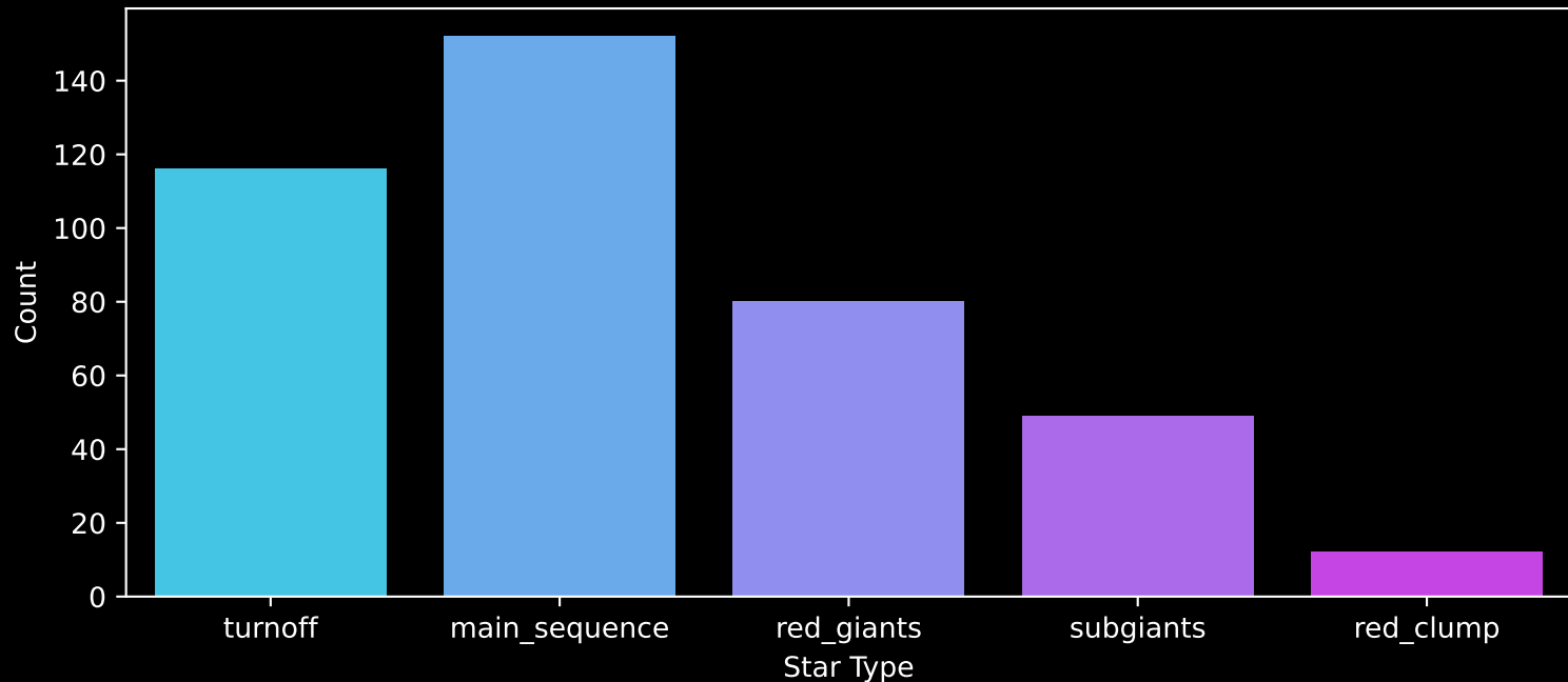
GALAH DR4 Field: [6584] Count plot of Star Type
