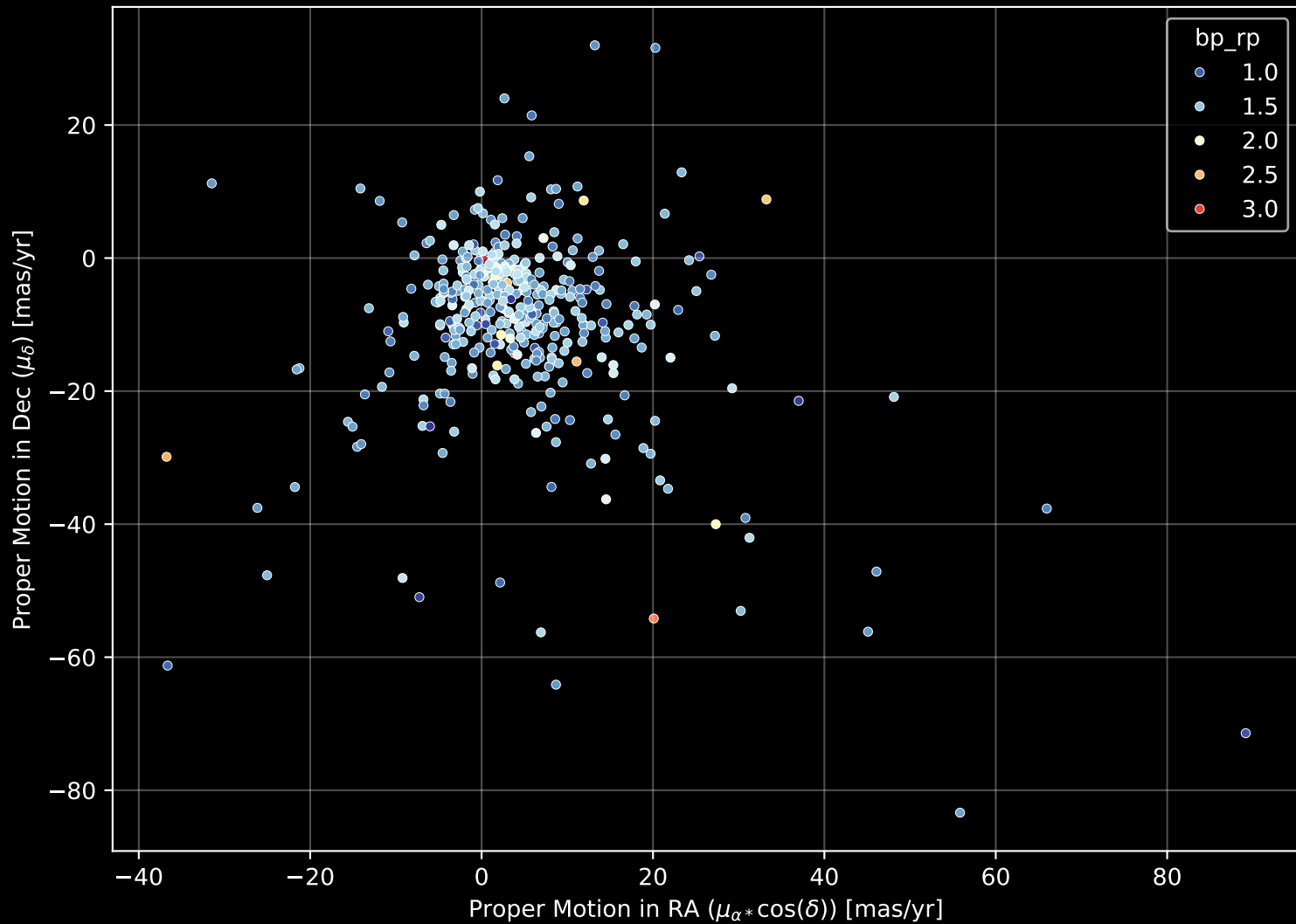
GALAH DR4 Field: [6584] Proper Motion Diagram (n= 409)
